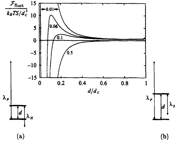
FIGURE 4 Fluctuation induced force in a hybrid cell as a function of the reduced thickness for various anchorings; \lambda_H/\lambda_P = 0.01, 0.06, 0.1 , and 0.5 . At small distances the fluctuation-induced force is attractive, \lambda_P > \lambda_H > d [inset (a)], then it becomes repulsive, \lambda_P > d > \lambda_H [inset (b)], and diverges at the transition ( d = d_c = \lambda_P - \lambda_H ).
